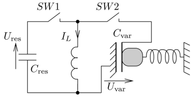
Fig. 4. Conditioning circuit for electrostatic transducer implementing a charge-constant energy conversion (Fig. 5) [11].
